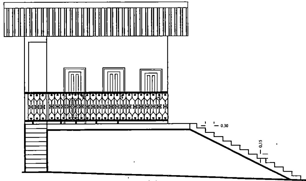
FRONT ELVATION
